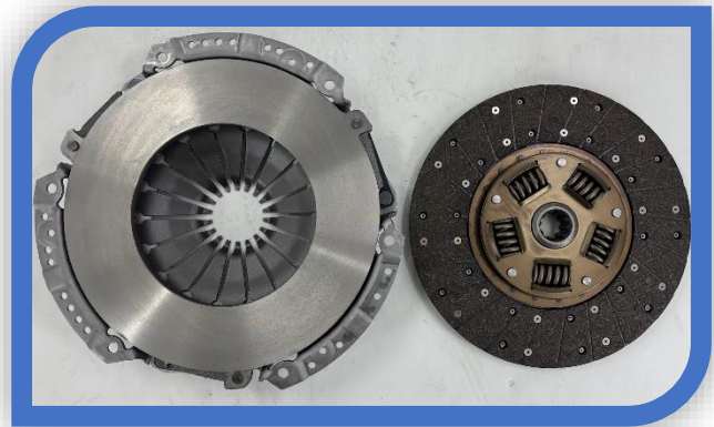
Aftermarket Wide Plate Design
